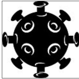
Virus
